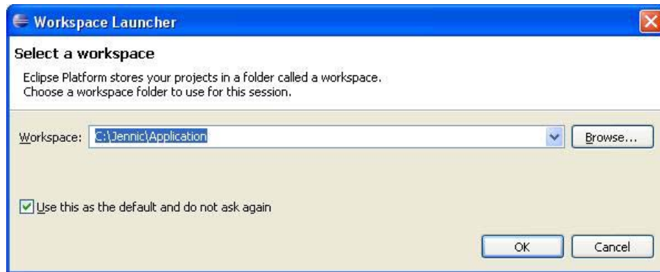
Figure 10: Workspace Launcher
