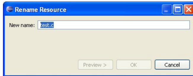
Figure 25: Rename Resource
